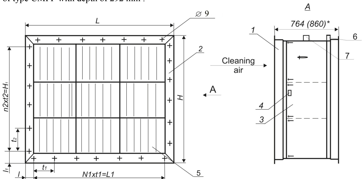
Fig. 1 Scheme of the filtering chamber of type FCCF.
